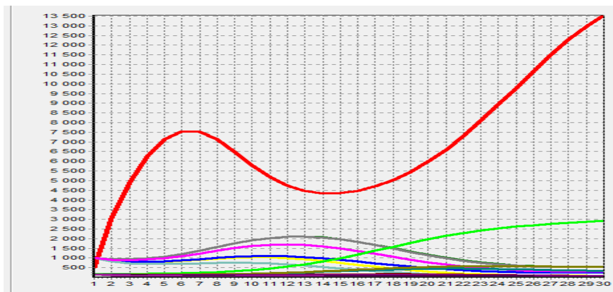
Расми 4.2.10. Ҳангоми \text{gam1}=0.021 , \text{gam2}=2.3 , K_0=0.0003 , N_0=500 , \text{tau}=0.01 , h1=0.1 , h2=0.1 , p=1 , q=6 .
