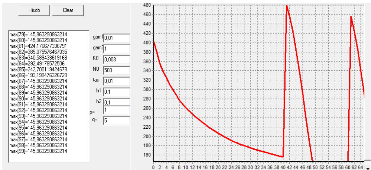
Расми 4.2.11. Ҳангоми \text{gam1}=0.01 , \text{gam2}=1 , K_0=0.003 , N_0=500 , \text{tau}=0.01 , h_1=0.1 , h_2=0.1 , p=1 , q=5 .
