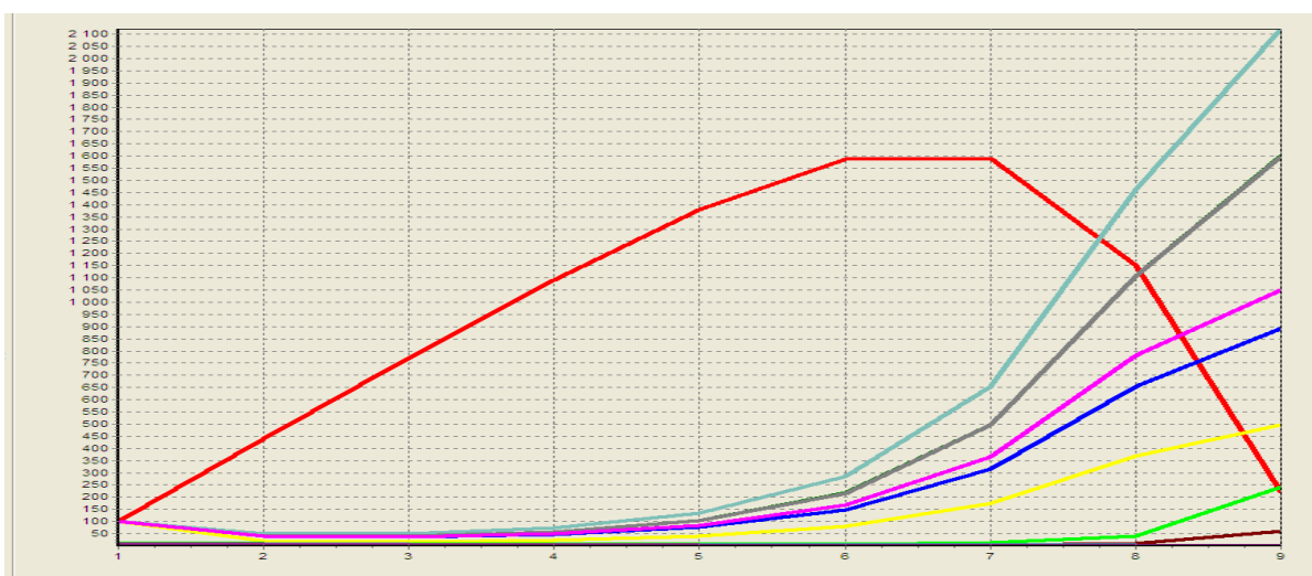
Расми 4.2.12. Ҳангоми \text{gam1}=0.02 , \text{gam2}=3 , K_0=0.0003 , N_0=500 , \text{tau}=0.01 , h_1=0.1 , h_2=0.1 , p=1 , q=4 .
