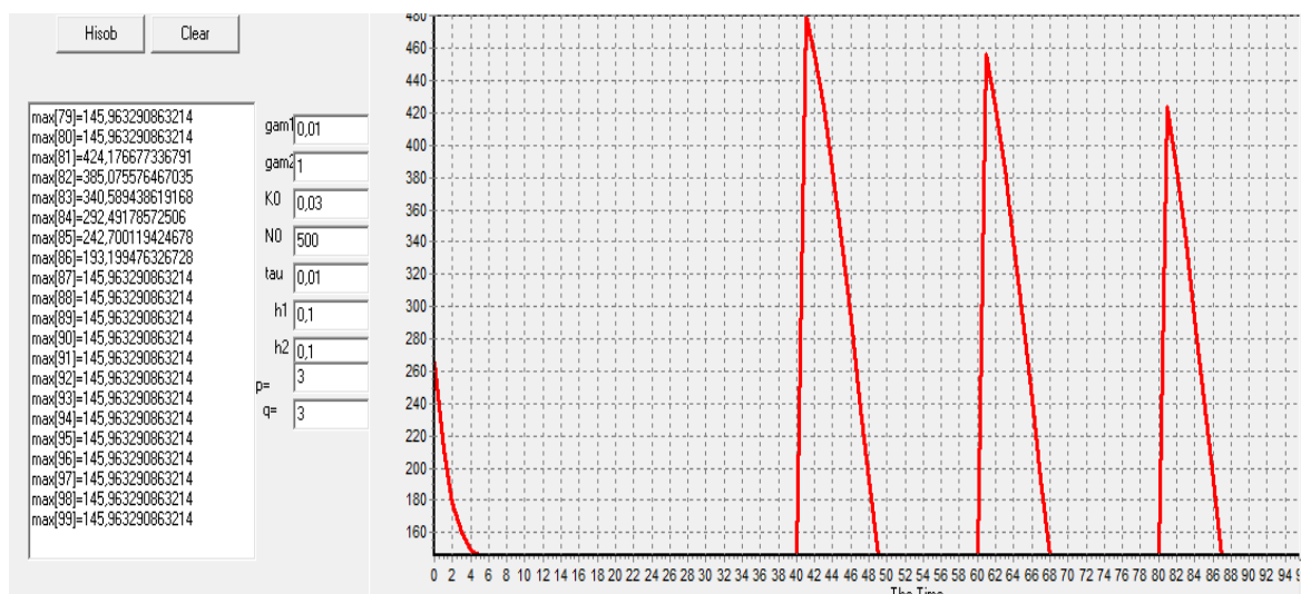
Расми 4.2.23. Ҳангоми \text{gam1}=0.01 , \text{gam2}=1 , K_0=0.03 , N_0=500 , \text{tau}=0.01 , h_1=0.1 , h_2=0.1 , p=3 , q=3 .
