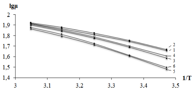
Рисунок 5. – Температурные зависимости молярной электропроводности \lg \mu от 1/T , 1- [\text{Ag}(\text{C}_7\text{H}_6\text{N}_2\text{S})(\text{H}_2\text{O})_3]\text{NO}_3 ; 2- [\text{Ag}(\text{C}_7\text{H}_6\text{N}_2\text{S})_2(\text{H}_2\text{O})_2]\text{NO}_3 ; 3- [\text{Ag}(\text{C}_7\text{H}_6\text{N}_2\text{S})_2\text{Cl}] ; 4- [\text{Ag}(\text{C}_7\text{H}_6\text{N}_2\text{S})_2\text{Br}] ; 5- [\text{Ag}(\text{C}_7\text{H}_6\text{N}_2\text{S})_2(\text{H}_2\text{O})_2]\text{SO}_4 и 6- [\text{Ag}(\text{C}_7\text{H}_6\text{N}_2\text{S})_2(\text{H}_2\text{O})\text{SCN}]
